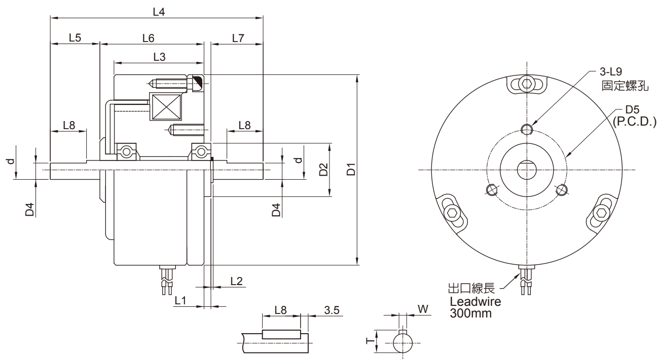
[CHB020AA軸端尺寸] [CHB020AA Shaft Dimensions]
